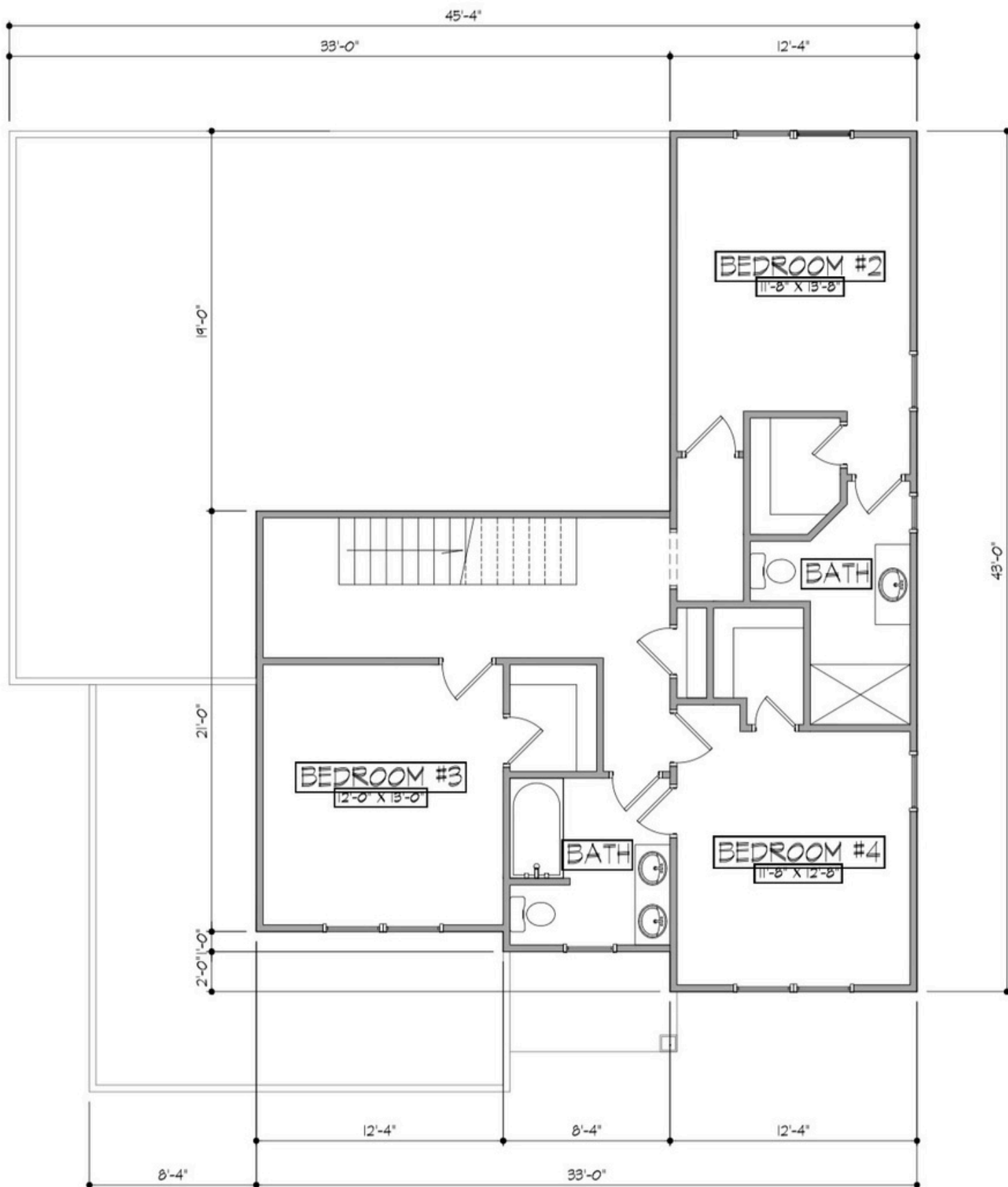
SECOND FLOOR PLAN 1/4" = 1'-0"
